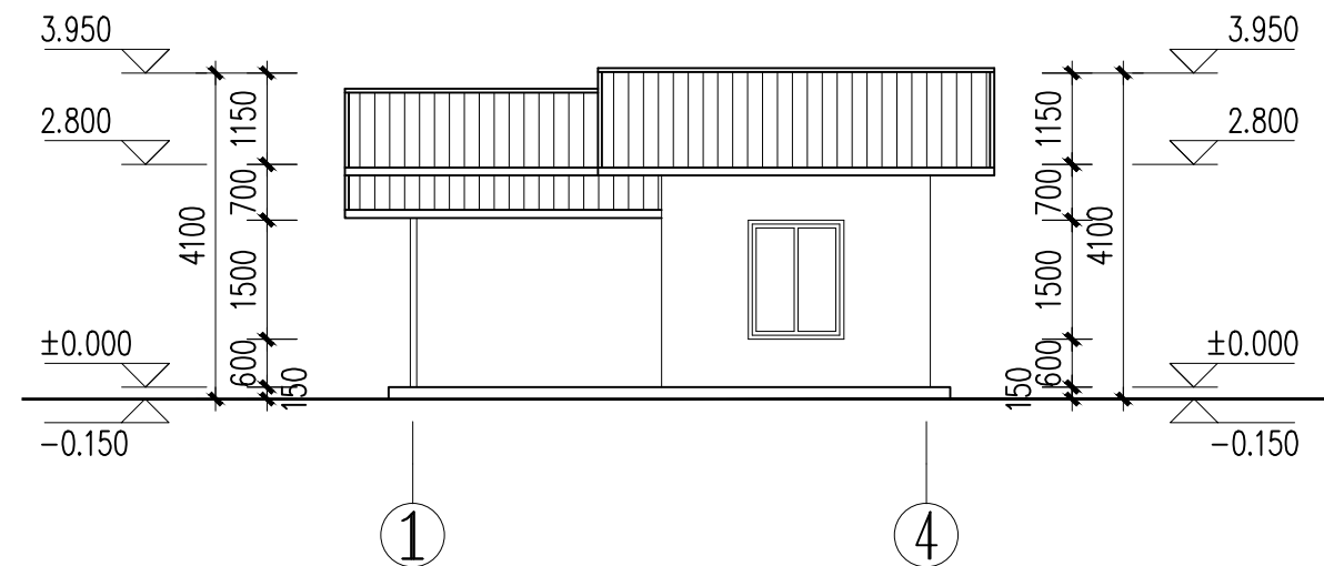
1-4 Axis Elevation 1:100
