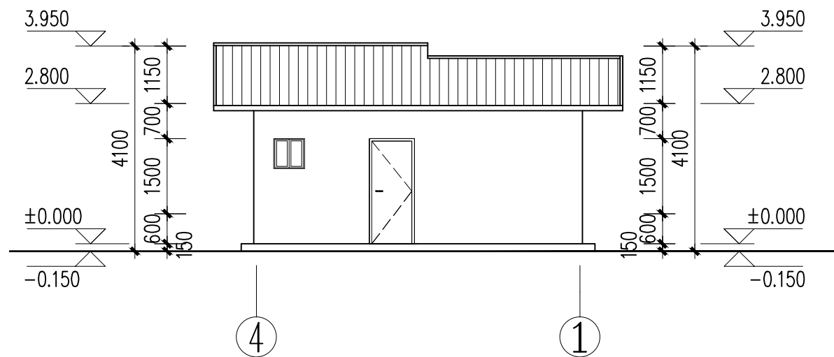
4-1 Axis Elevation 1:100
